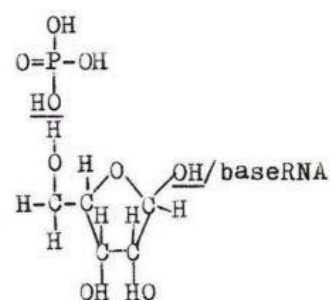
ribose sugar \text{C}_5\text{H}_{10}\text{O}_5
