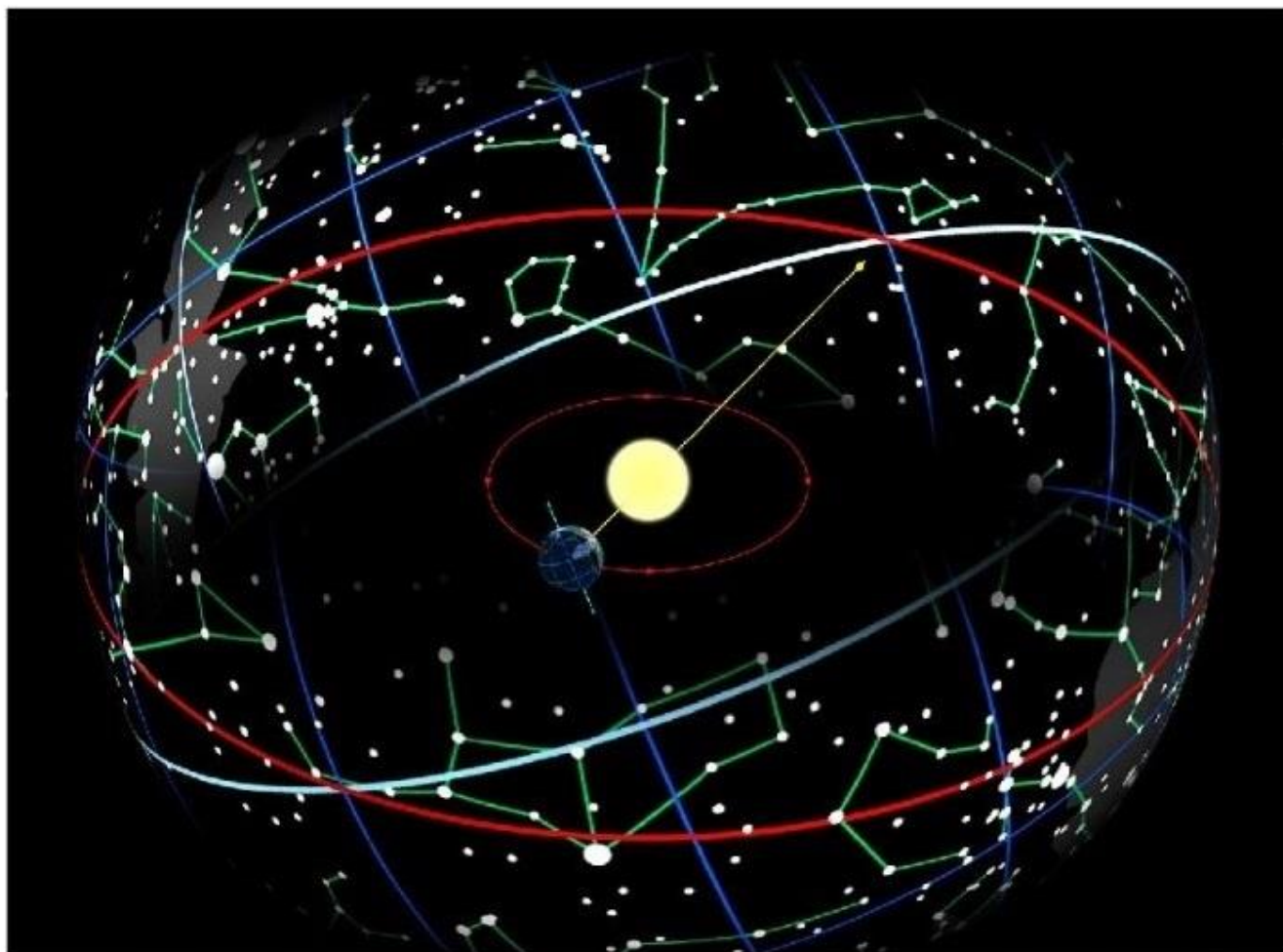
The Earth in its orbit around the Sun causes the Sun to appear on the celestial sphere moving along the ecliptic (red), which is tilted 23.44^\circ with respect to the celestial equator (blue-white).
